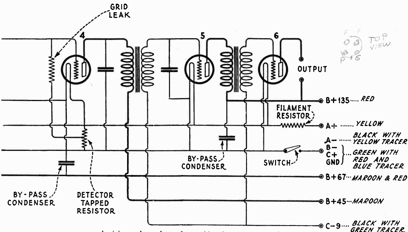
and wiring color scheme for making battery connections
